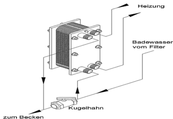
Bypass -Prinzip
